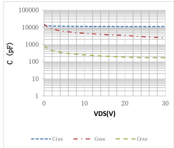
Fig.2 Capacitance Characteristics
