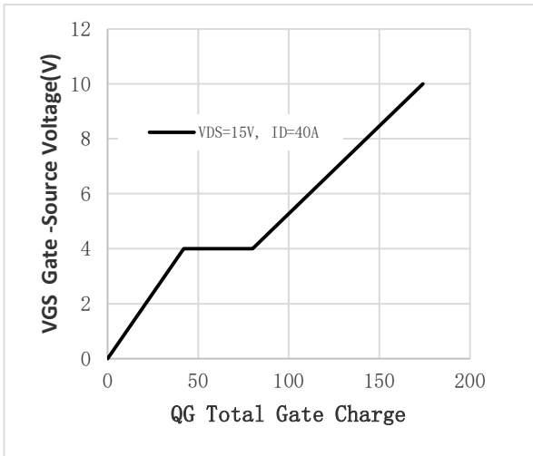
Fig.1 Gate-Charge Characteristics
